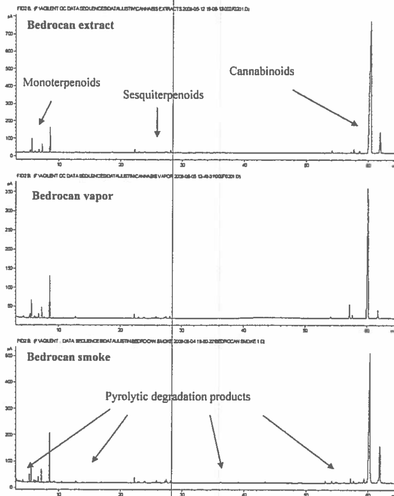
Fig. 1. Typical GC-FID Chromatograms of a Bedrocan® Extract, Vapor and Smoke Sample
